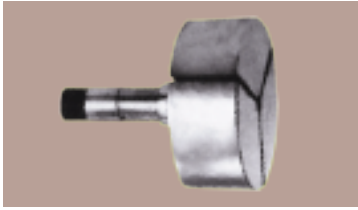
.637"-26 External Thread, Soft head for machining to specific requirements
